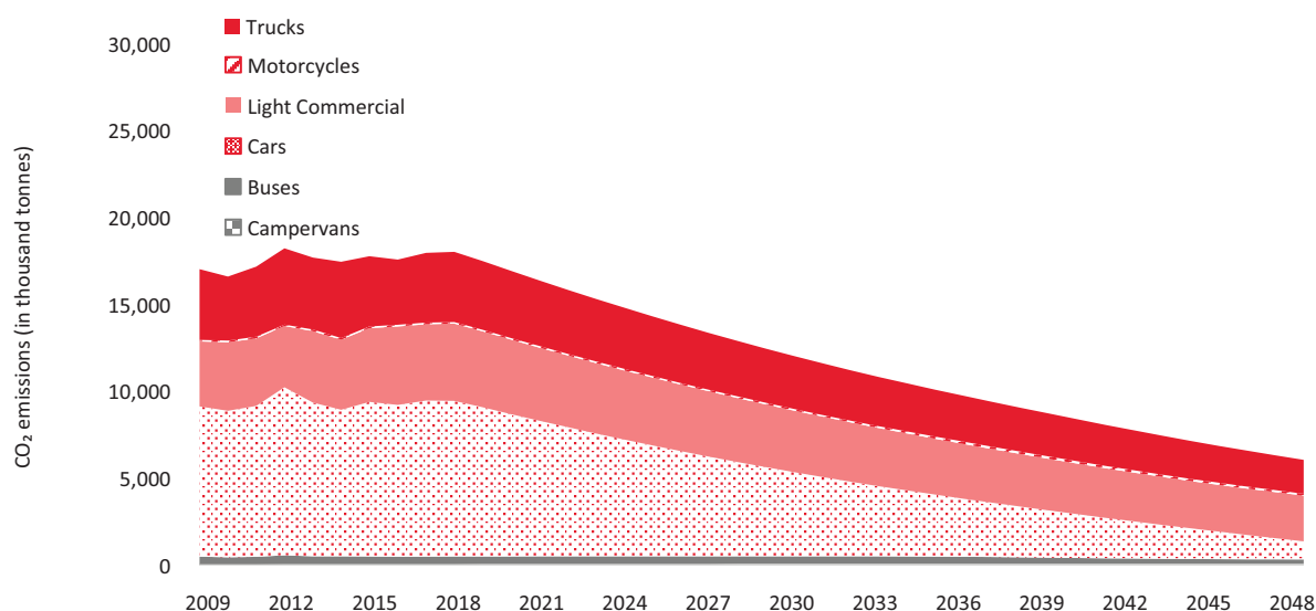
Figure 132. Time series of modelling projections of greenhouse gas emissions across the road vehicle fleet by vehicle type projected out to 2048 under Cruise Control scenario
