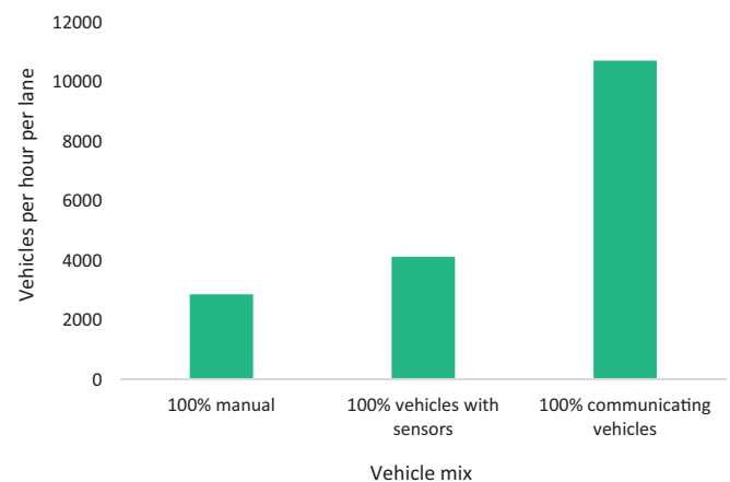
Figure 13. Highway capacity under full-adoption scenarios for manual, sensor-equipped and communicating vehicles
