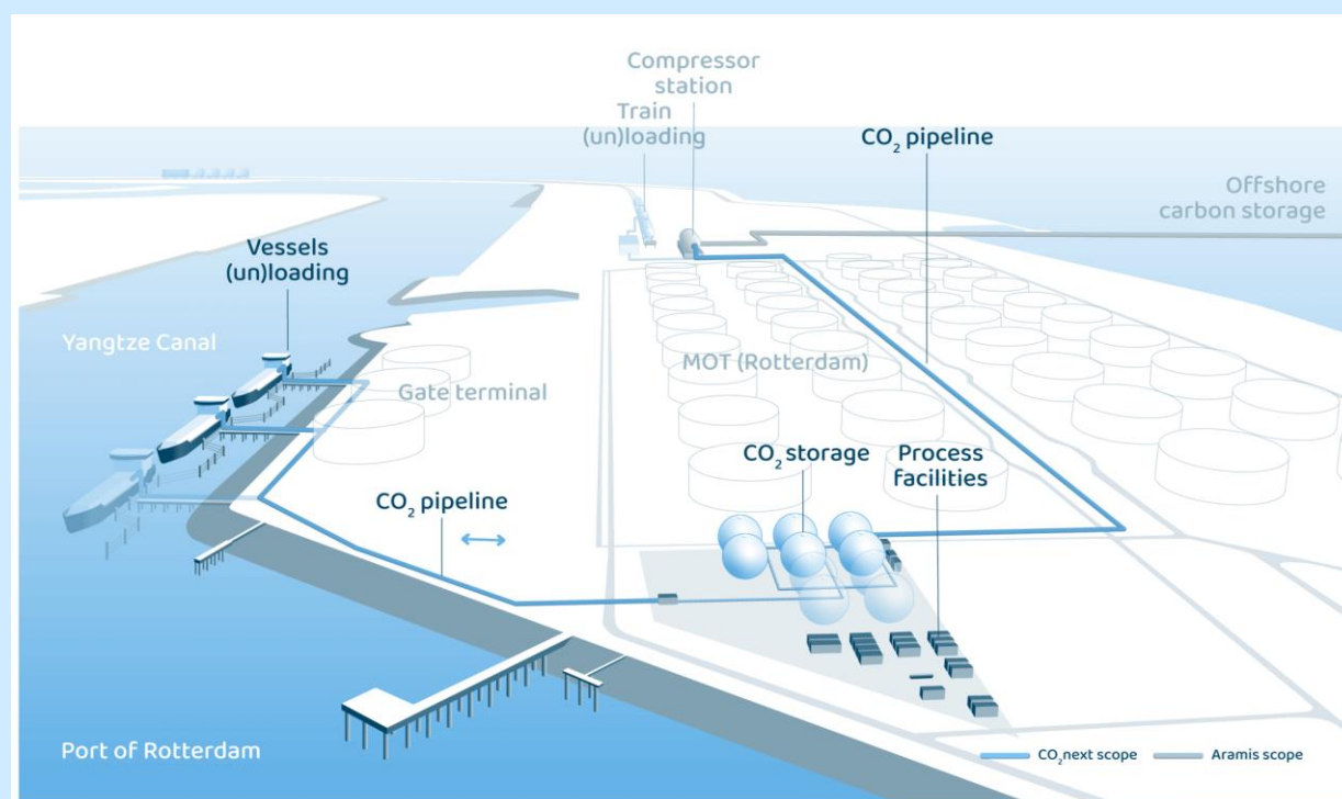
Figure 7: Schematic of the CO 2 next CO 2 import-export facility
