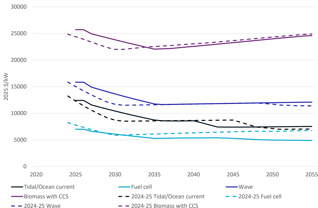
Figure 4-18 Projected technology capital costs under the Global NZE by 2050 scenario compared to 2024-25 projections
